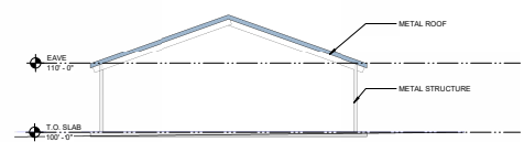
SHOOT HOUSE ELEV SW 1/8" = 1'-0"
