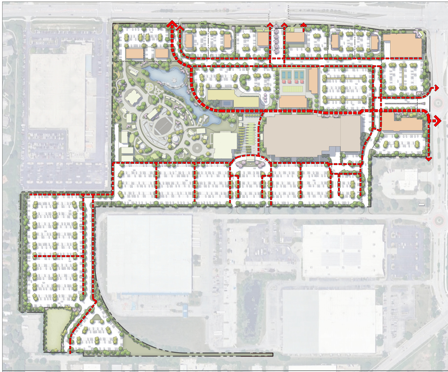
SITE PLAN 1" = 100' 0 100 200 300
