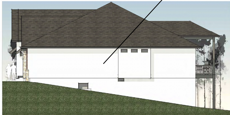
3 Right Elevation Color 3/16" = 1'-0"
