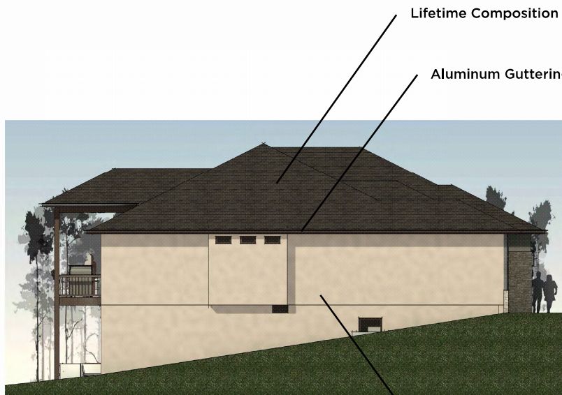
2 Left Elevation Color 3/16" = 1'-0"
