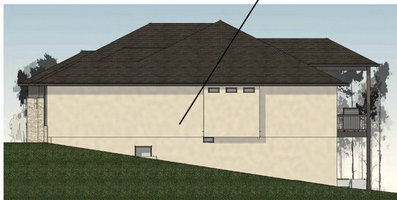
4 Right Elevation Color 3/16" = 1'-0"
